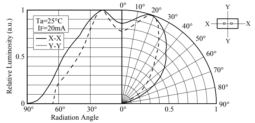
■ Directivity (NSPGF50S)
